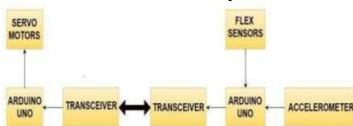
Fig. 1: Block diagram of Robotic arm
